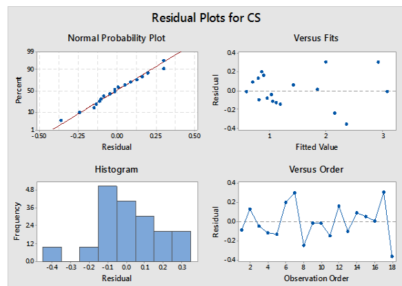
Fig: 4. Residual Plots for Cutting Speed
