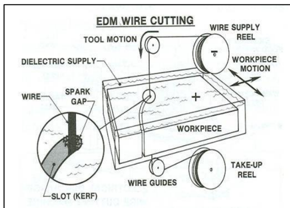
Fig. 1. Principal of WEDM [10]
