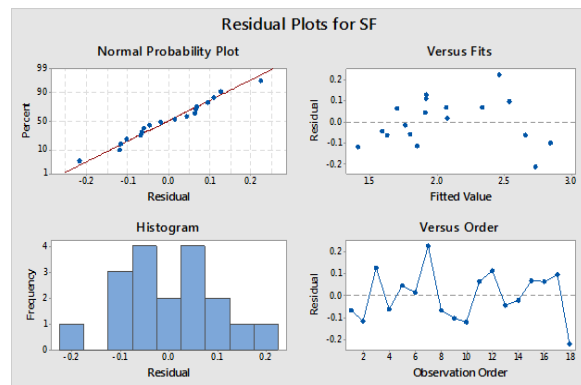
Fig: 7. Residual Plots for Surface finish
