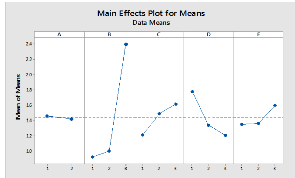
Fig: 3. Effects of Process Parameters on Cutting Rate (S/N data)
